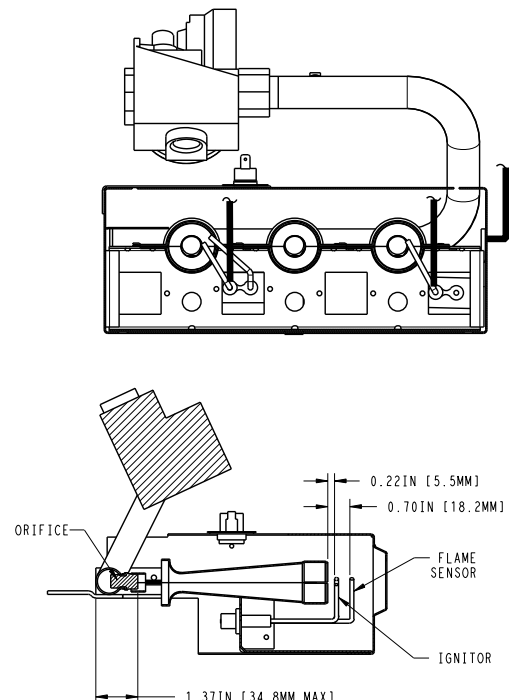
Fig. 3 – Single-Stage Igniter, Flame Sensor; Orifice/Main Burner Relationship
