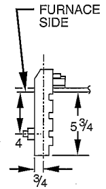
FRONT VIEW
