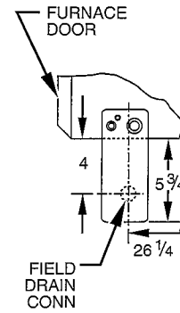
END VIEW
