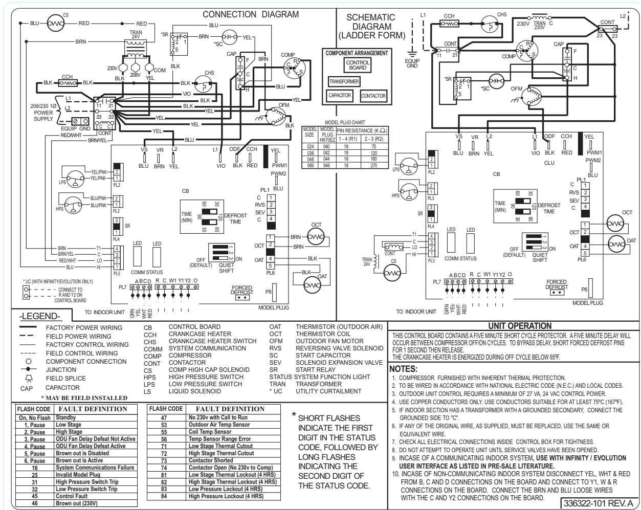
Fig. 1 – Wiring Diagram — Model sizes 2 - 5 tons, 208/230-1
