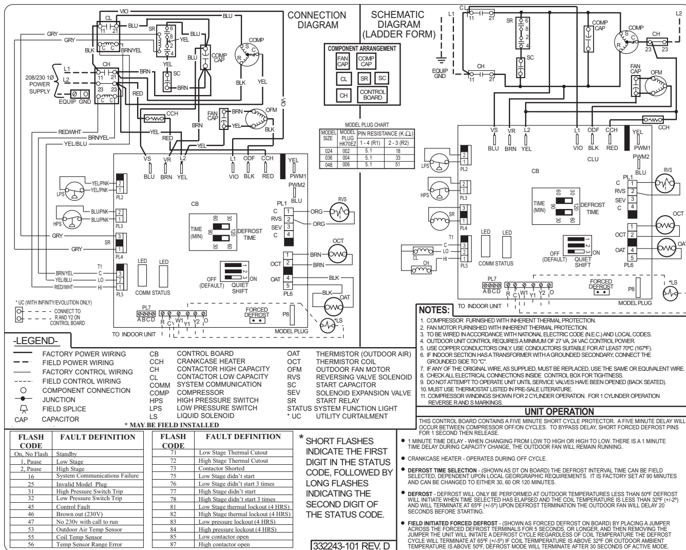
Fig. 1 – Wiring Diagram — Model sizes 2-4 tons, 208/230-1
