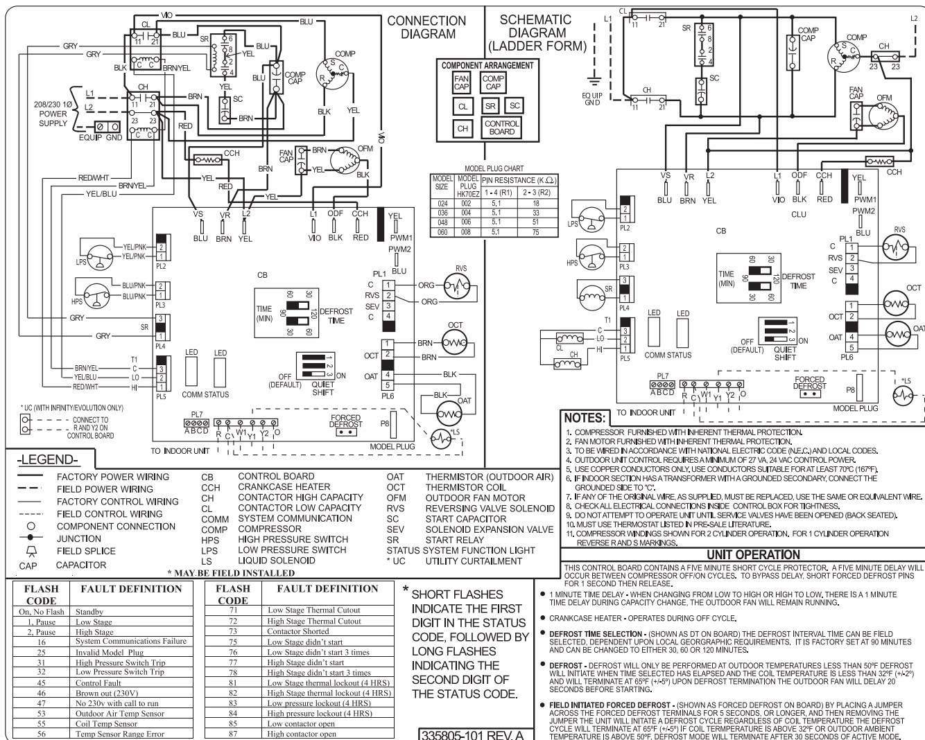
Fig. 1 – Wiring Diagram — Model size - 5 tons, 208/230-1
