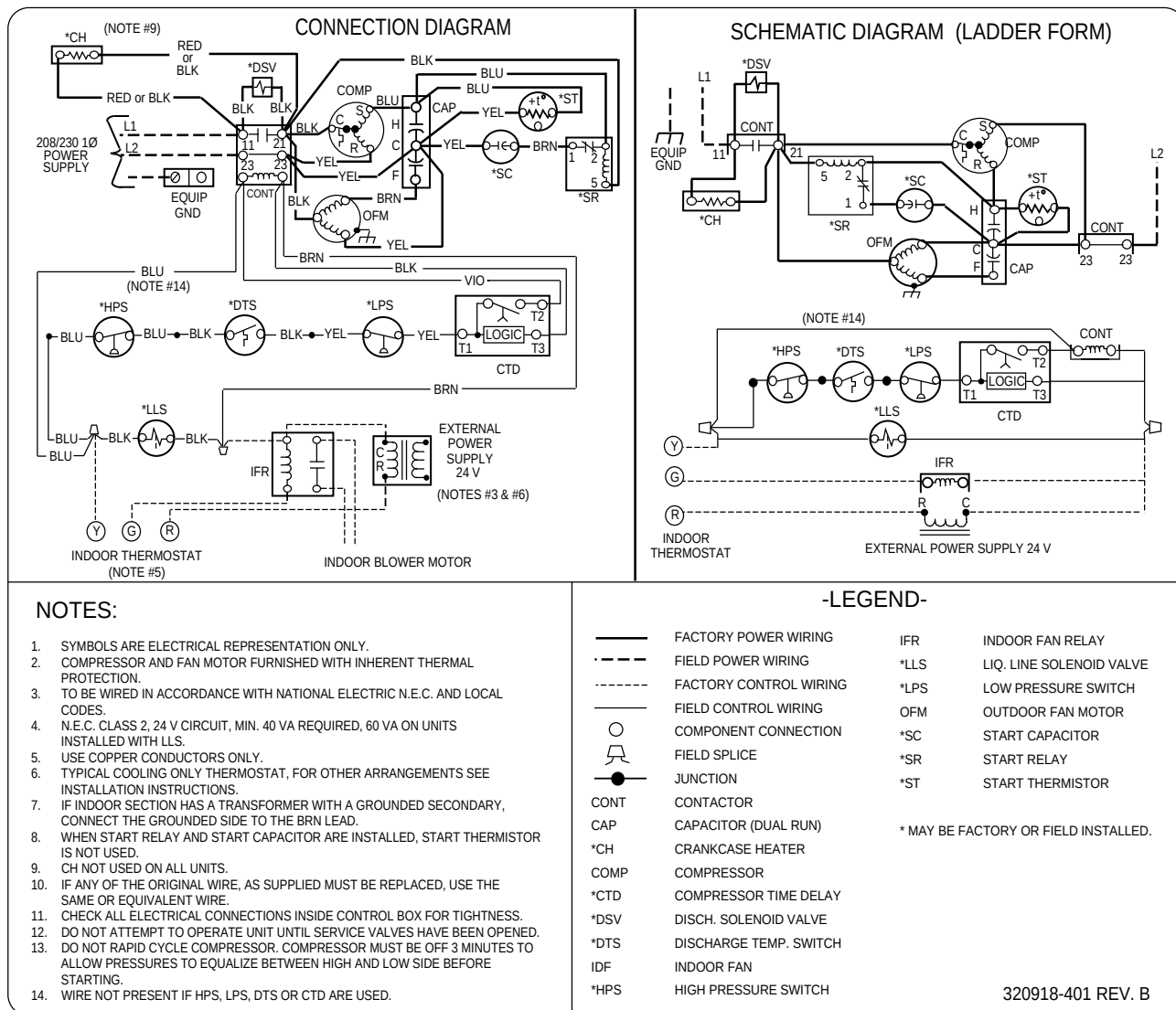
Fig. 1—38TRA018(0,1); 024-030(1,2); 036-048(1,3); 208/230v, 1 Phase, 60 Hertz
