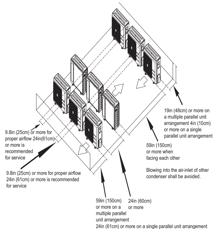
Fig. 7 – Multi-Unit Clearances
