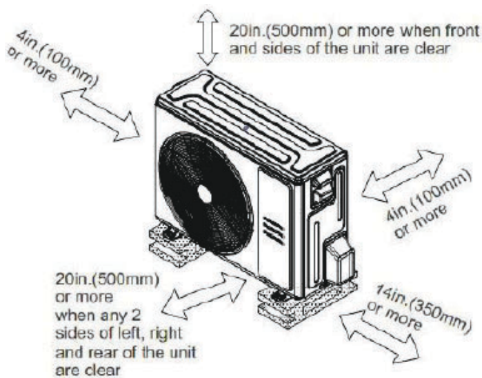
Fig. 6 – Clearances
