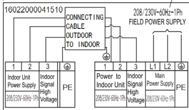
Fig. 8 – 9K/12K/18K/24K/30K/36K – 208/230V Connection Diagram
