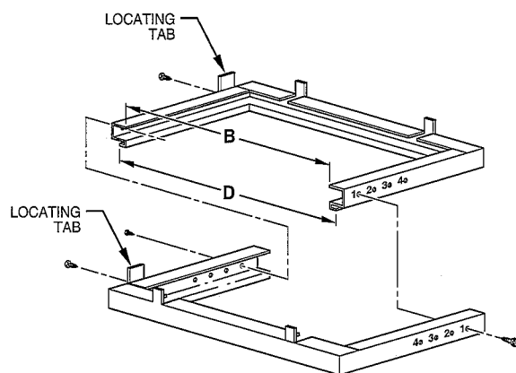
Disassembled
