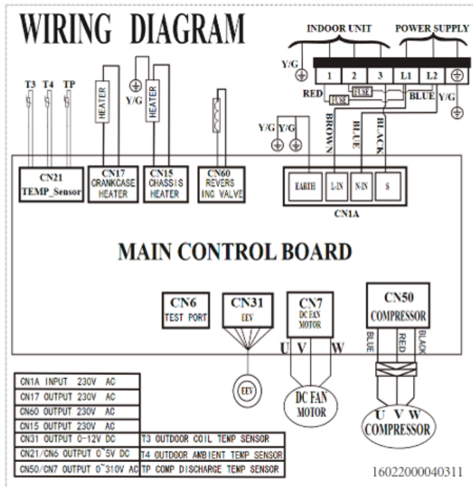
Fig. 9 – 9K/12K – 208/230V Wiring Diagram
