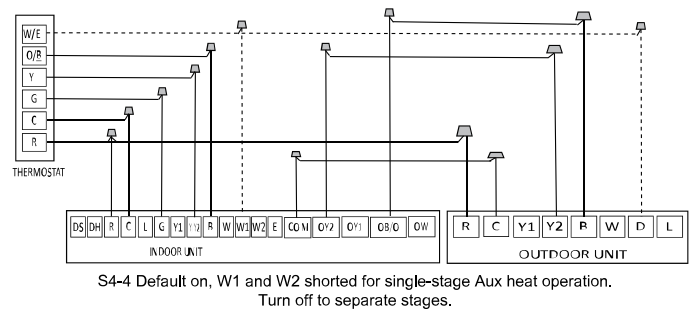
Fig. 15 – Wiring for 2H and 1C Thermostat
