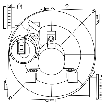
INDUCER ASSEMBLY
