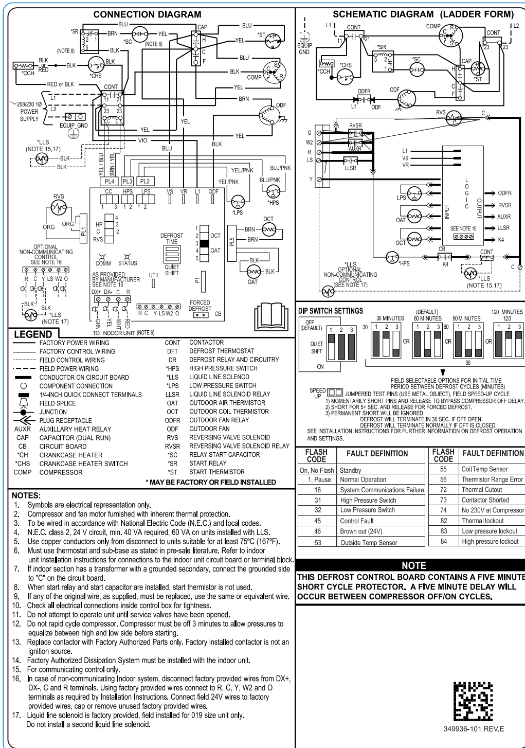
Fig. 1 – Size 1.5 - 5 Tons
