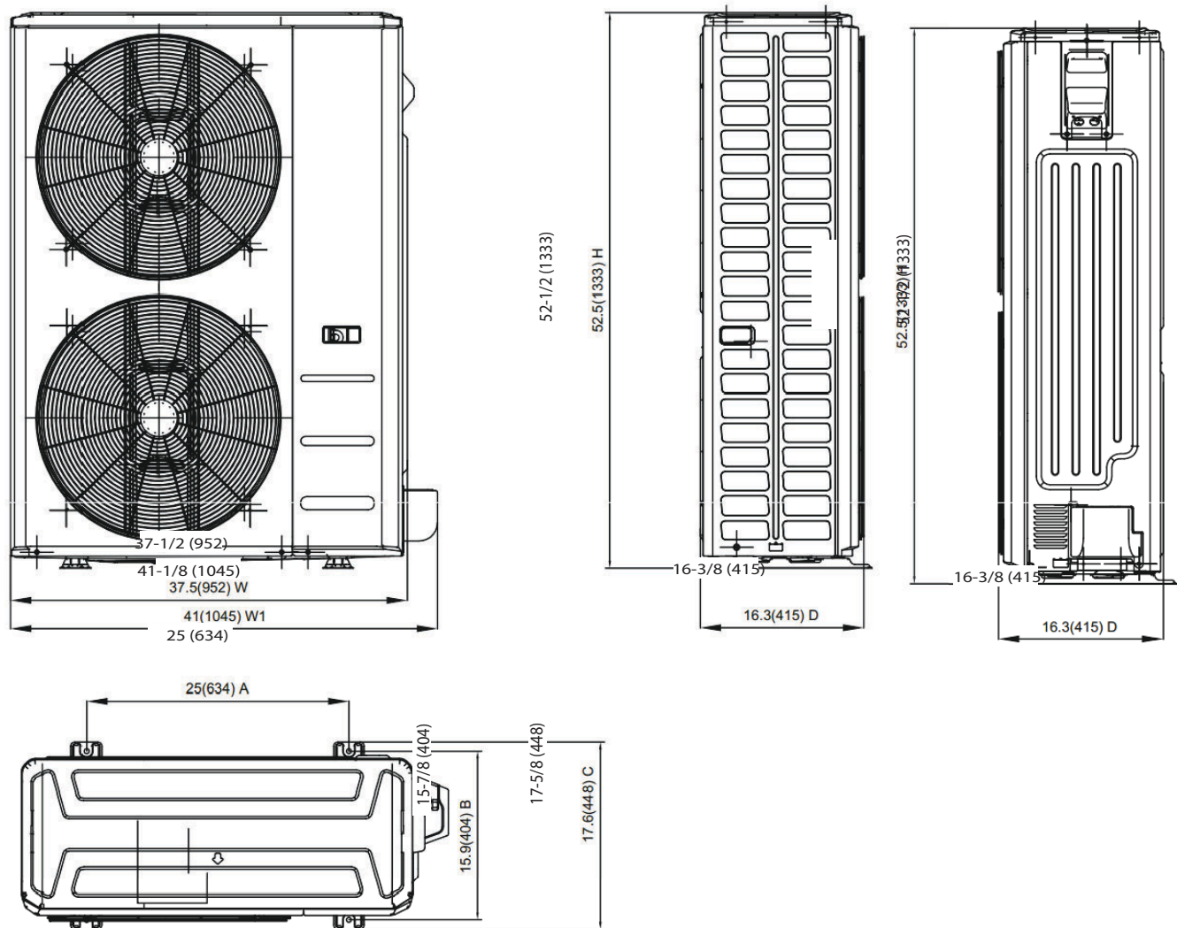
Fig. 4 – Outdoor Dimensions Size 48K and 58K
