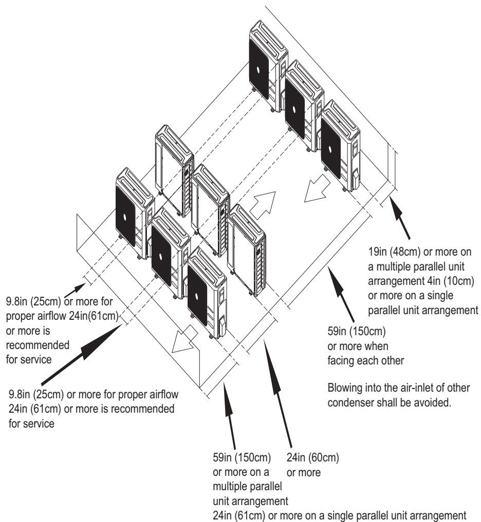
Fig. 6 – Clearances for Multiple Units
