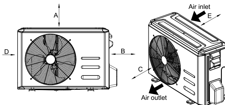
Fig. 5 – Clearances
