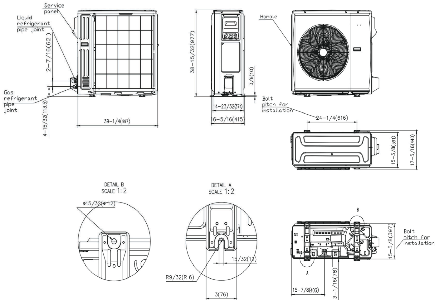
Fig. 3 – Outdoor Dimensions Size 36K
