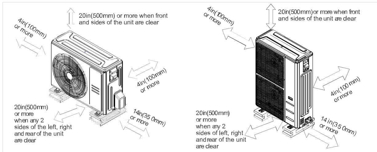
Fig. 6 – Clearances
