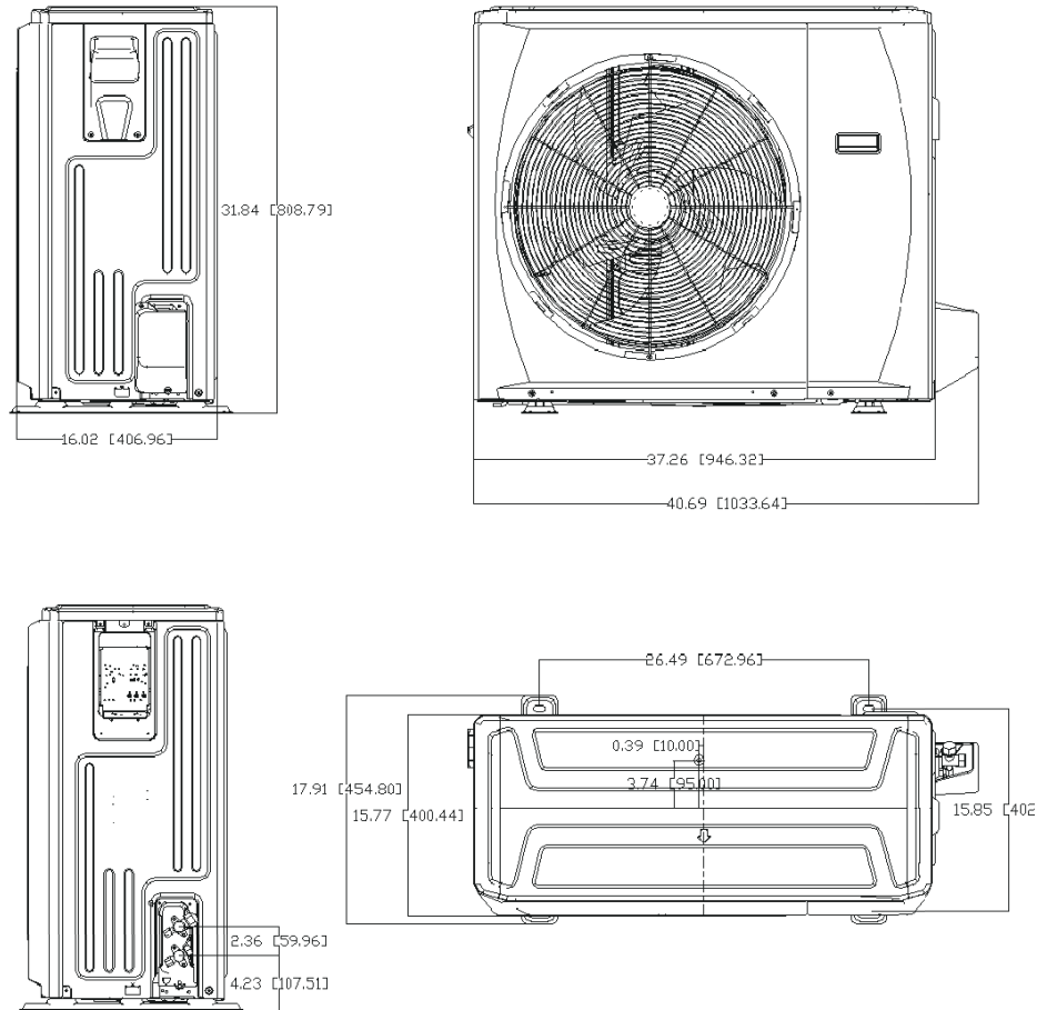
Fig. 4 – Sizes 30/36K
