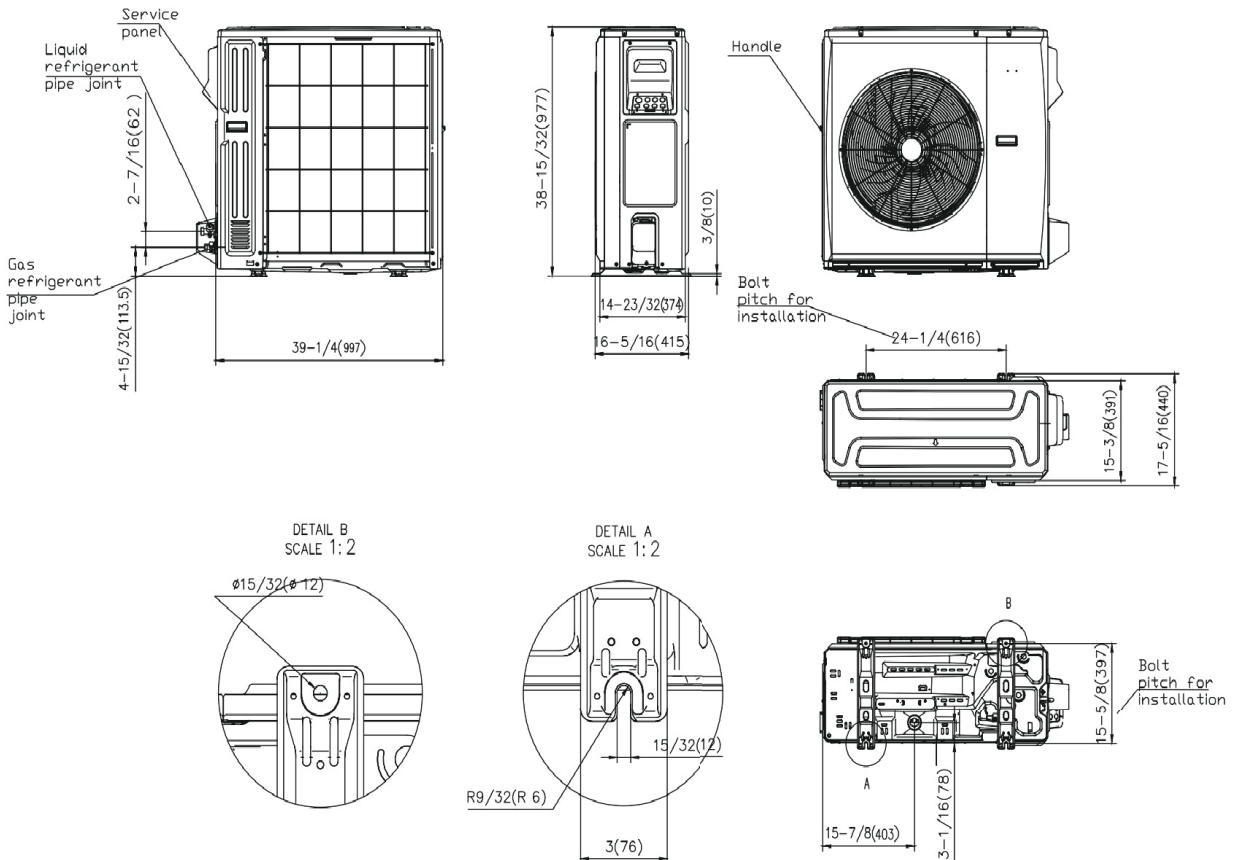
Fig. 5 – Sizes 48/60K
