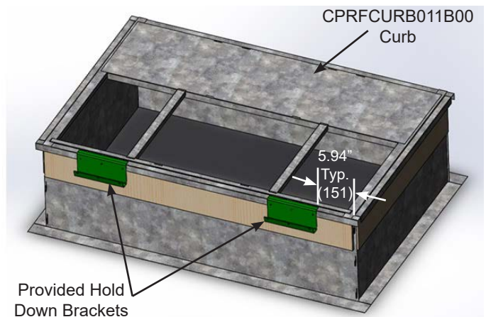
Fig. 5 - Hold Down Brackets For CPRFCURB011B00 Curb used with Large Cabinet Unit
