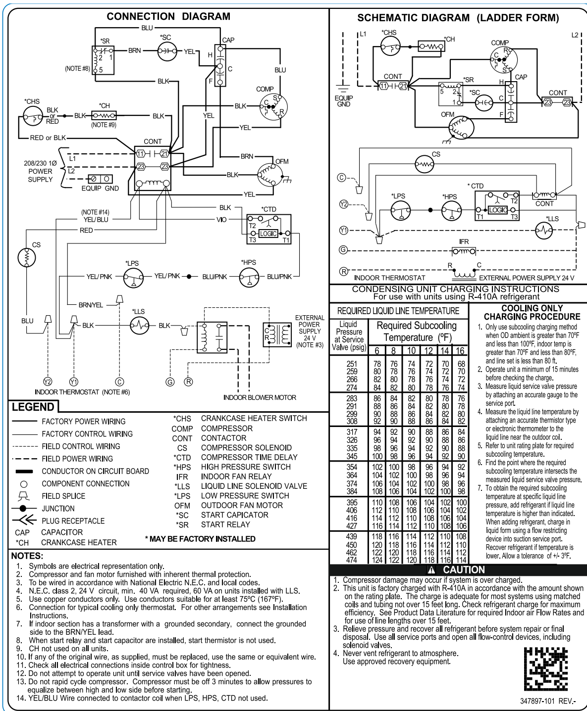
Fig. 1 – 24-60 Wiring Diagram
