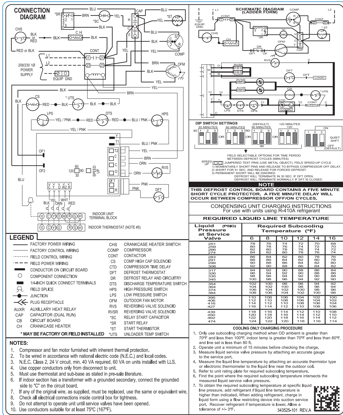
Fig. 1 – Wiring Diagram — Models BH17NA024-060, 208/230-1
