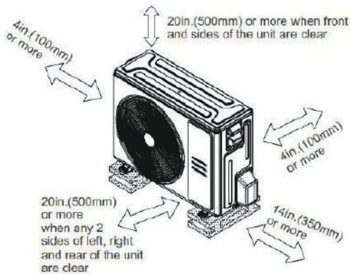
Fig. 6 – Clearances
