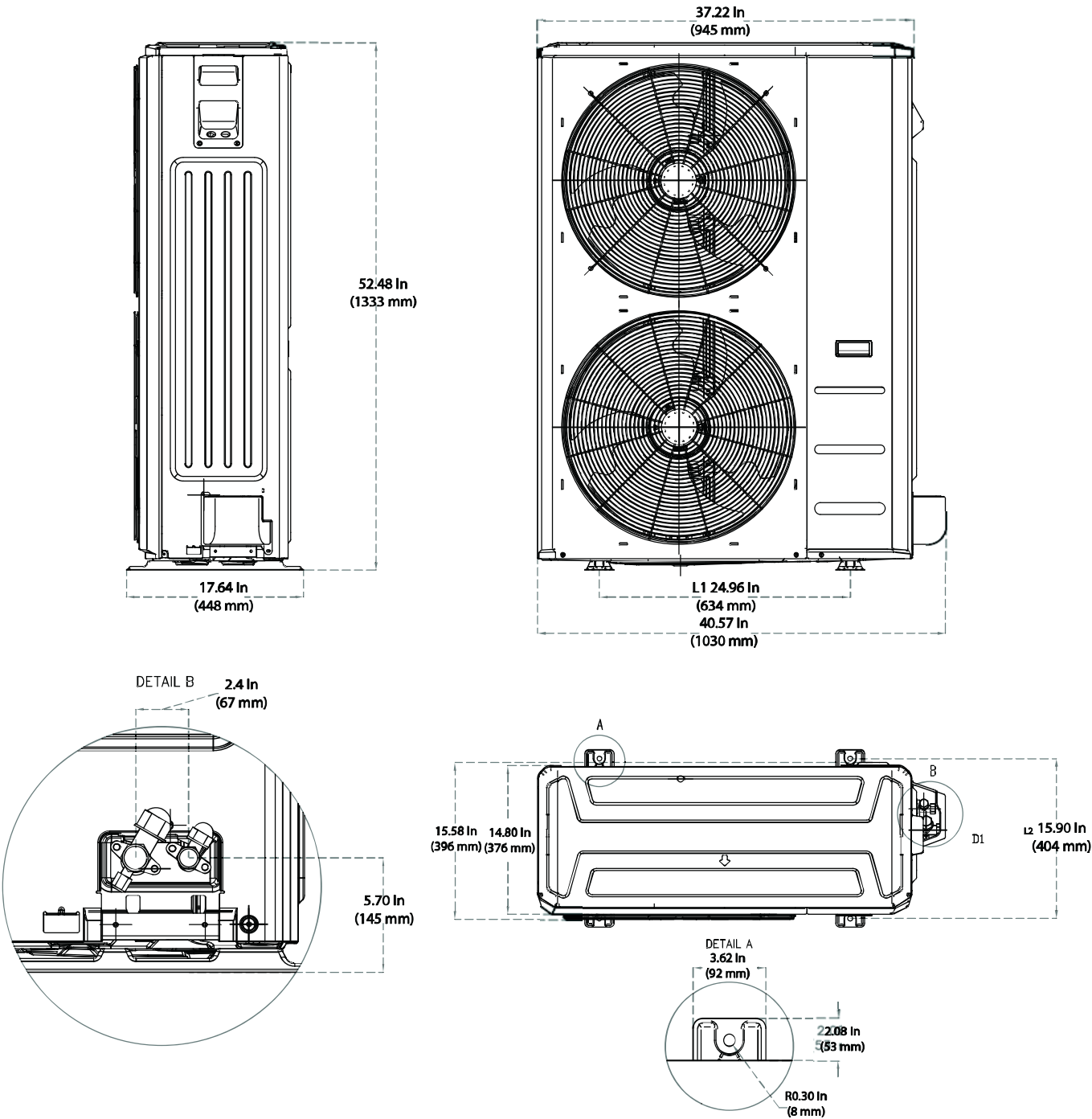
Fig. 4 — Outdoor Dimensions Size 48K - 58K
