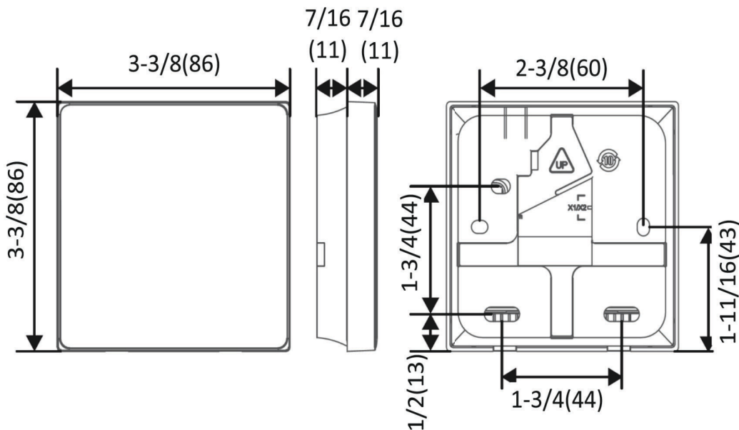
Fig. 2 – Dimensional Drawing
