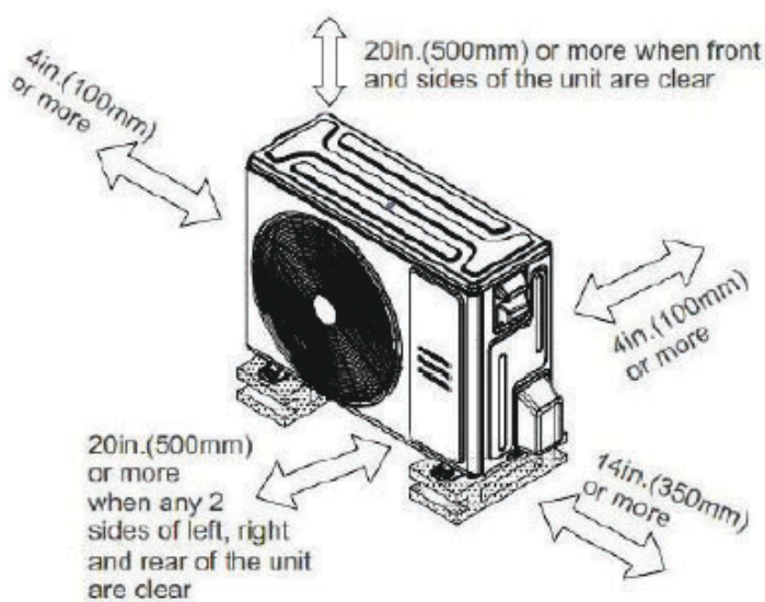
Fig. 6 – Clearances
