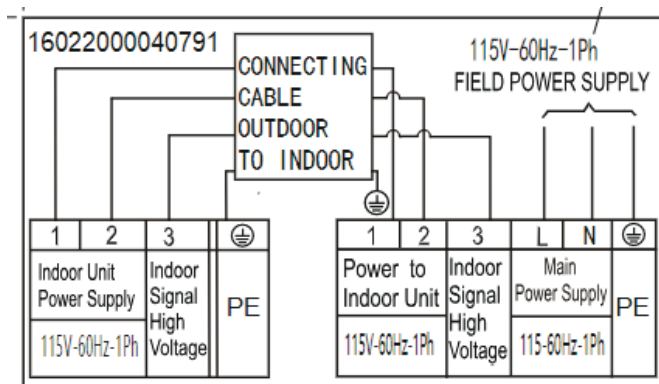
Fig. 7 – 12K – 115V Connection Diagram
