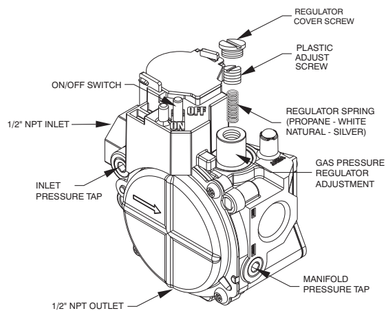
Fig. 14 - Single-Stage Gas Valve
