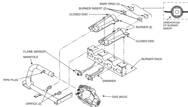
Fig. 7 - Two-Stage Orifice Installation
