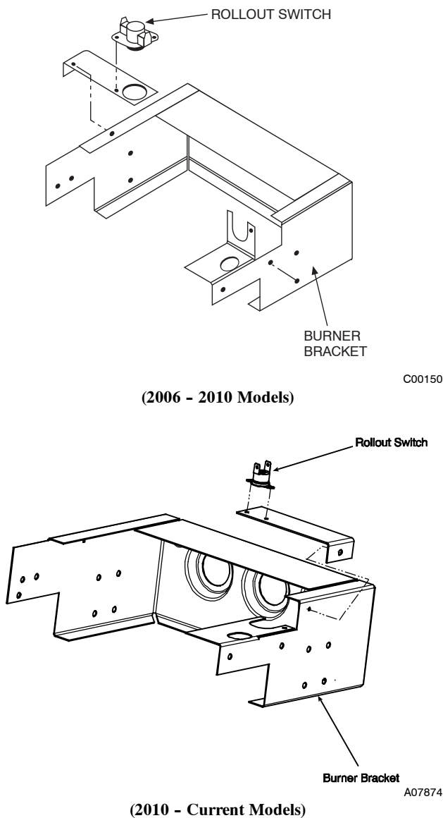
Fig. 3 - Two-Stage Burner Bracket
