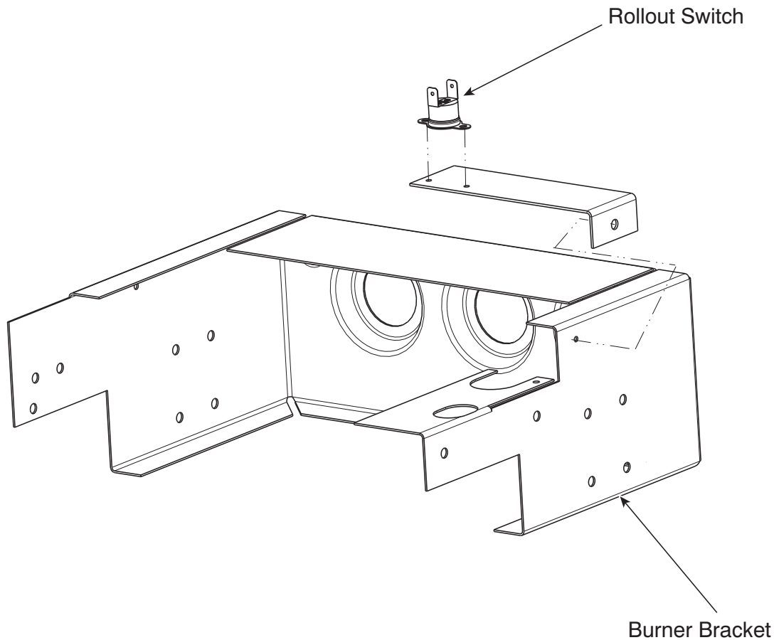
Fig. 12 - Single-Stage Burner Bracket
