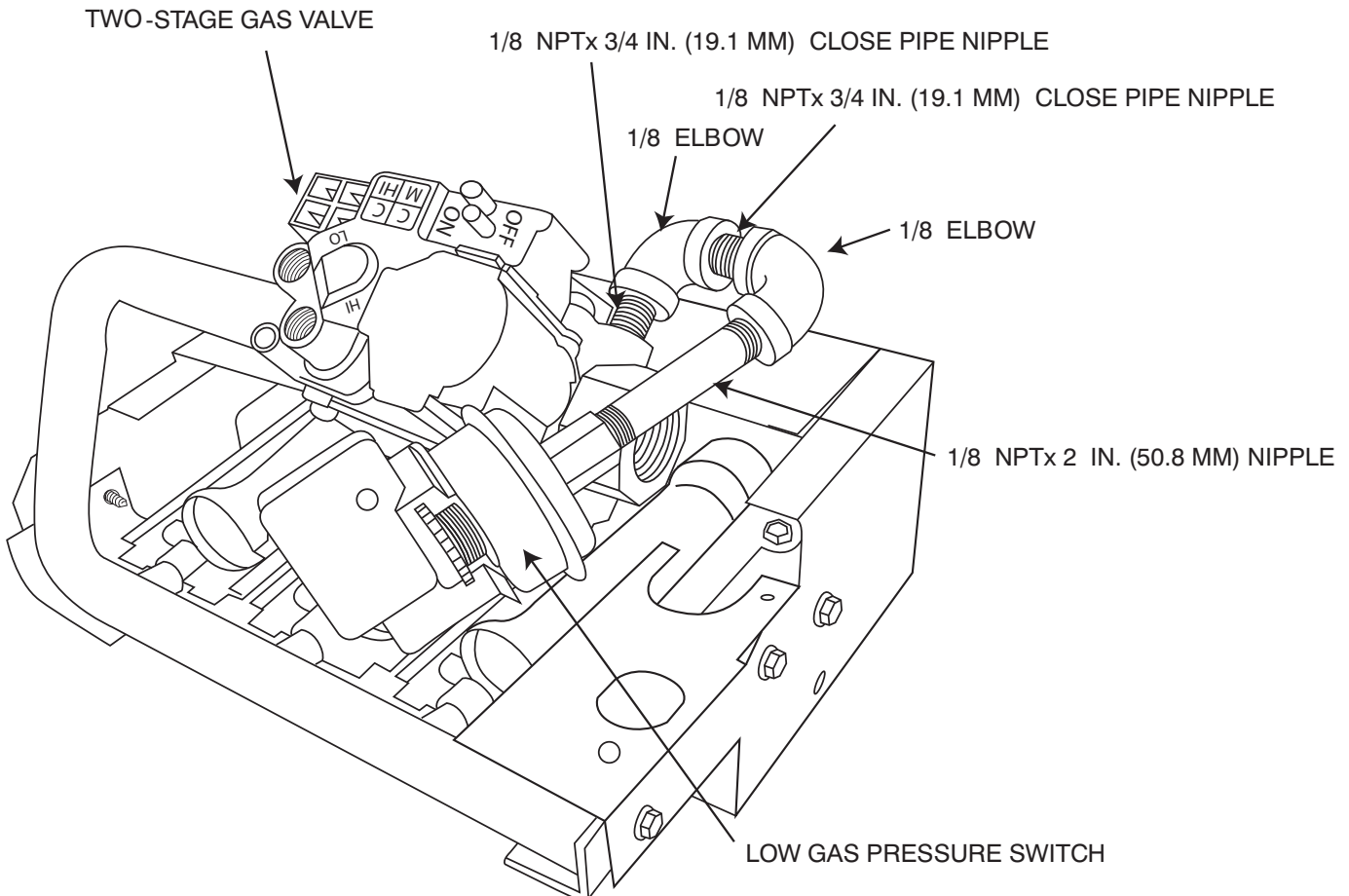
Fig. 11 - Installing Elbows, Nipples, and Pressure Switch on Two-Stage Units
