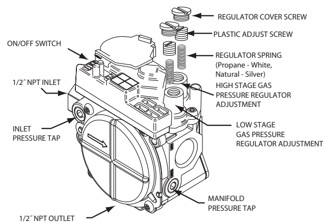
Two-Stage 36G Valve
