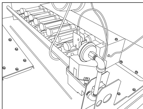
Fig. 5 - LP Pressure Switch Piping (36H Gas Valve Shown)
