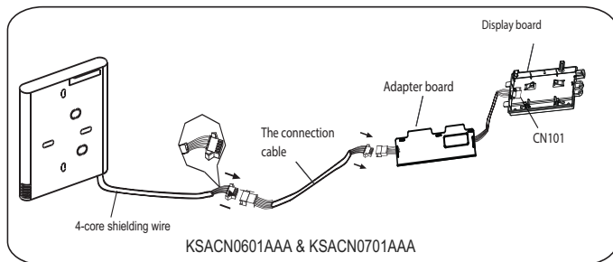
Fig. 10 — Installation of KSACN0601AAA and KSACN0701AAA
