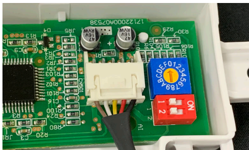
Fig. 20 — Adapter Board to Display Board Connection
