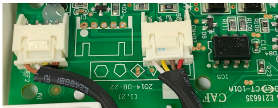
Fig. 21 — Wired Controller Port
