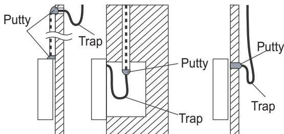
Fig. 8 — Seal the wires
