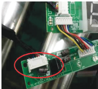
Fig. 14 — CN201 Connection to the Main Control Board
