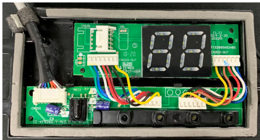
Fig. 18 — Display Board Installed on the Display Board Holder
