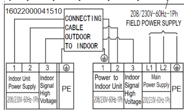
Fig. 8 – 9K/12K/18K/24K/30K/36K Connection Diagram
