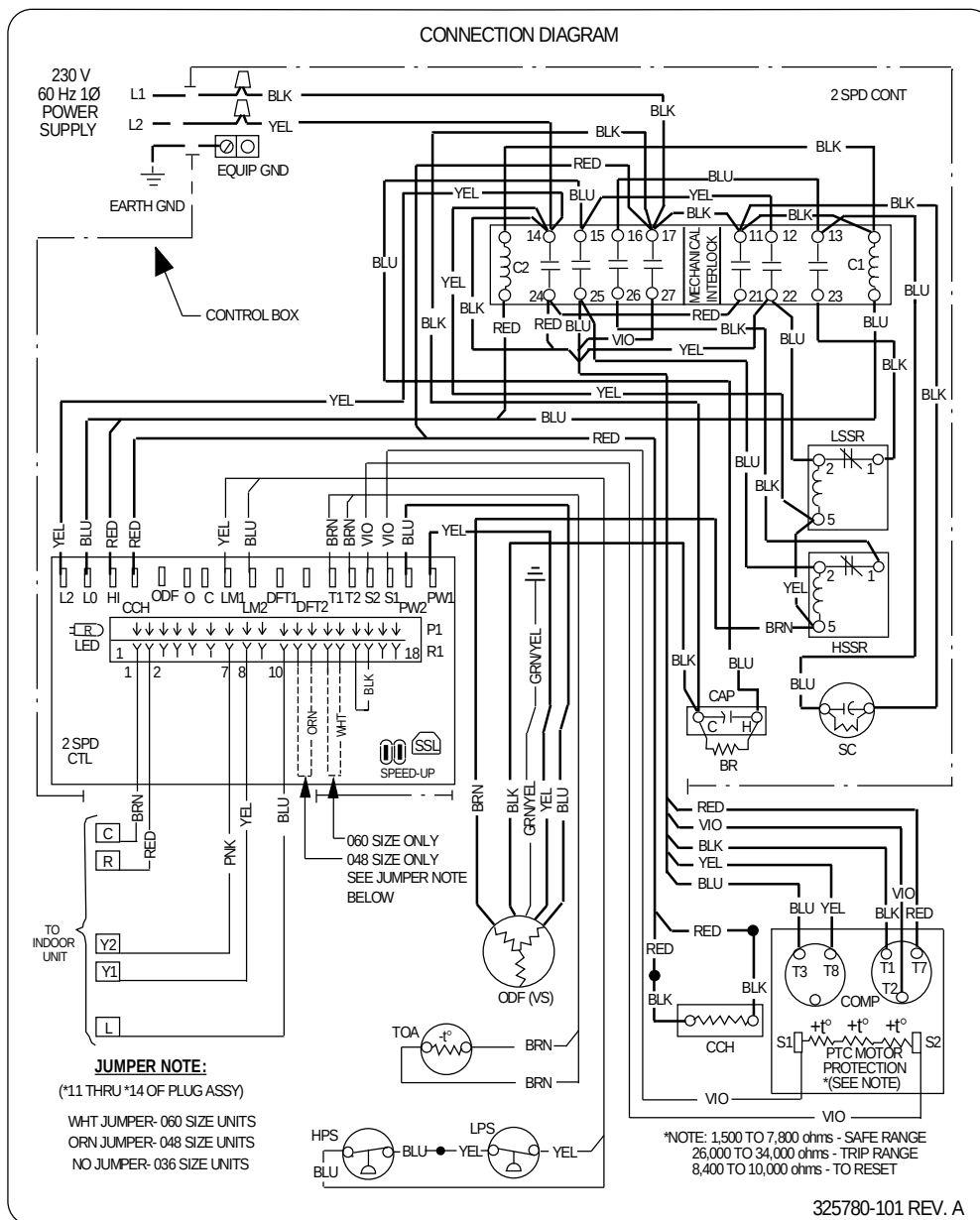
Fig. 2—38TDA036, 048, 060 208/230v, 1 Phase, 60 Hertz
