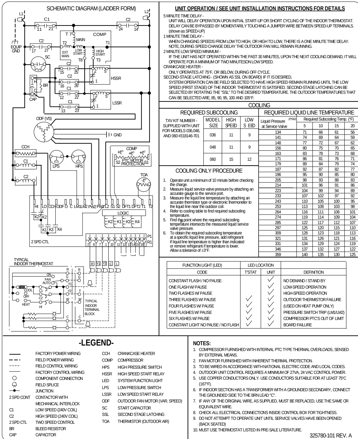
Fig. 1—38TDA036, 048, 060 208/230v, 1 Phase, 60 Hertz
