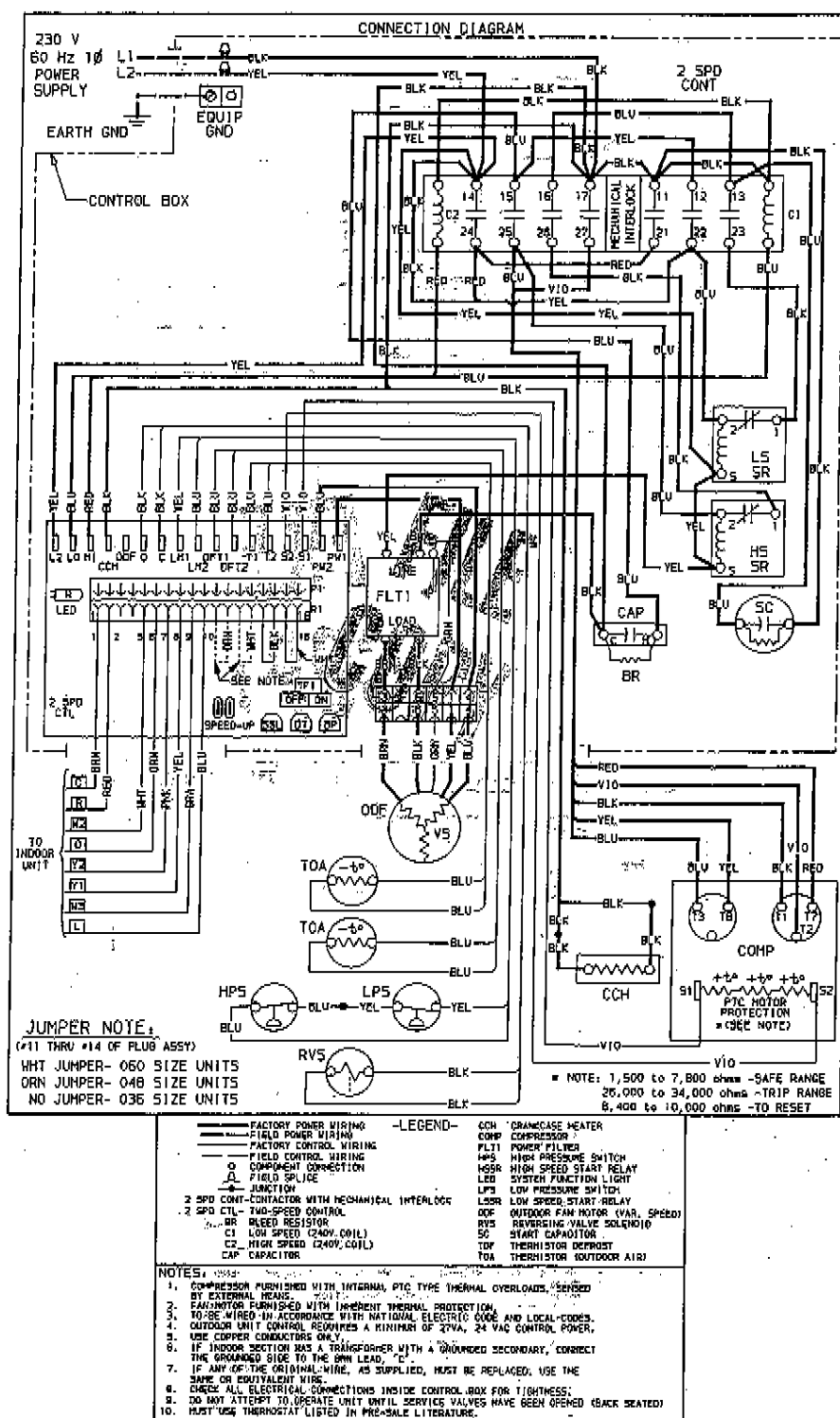
Fig. 1—38YD Connection Diagram (036, 048, and 060)
