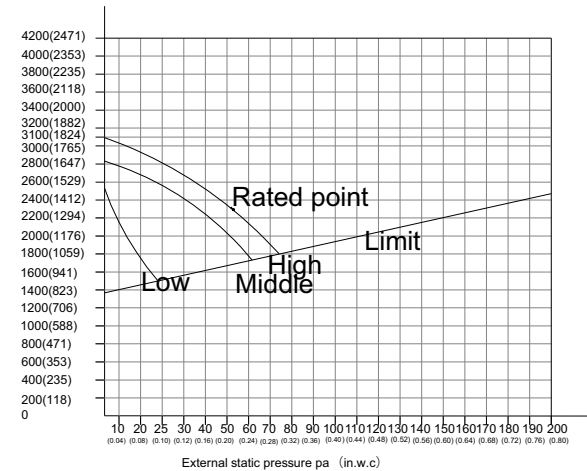
Air volume m3h(CFM) SP1
