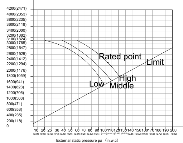
Air volume m3h(CFM) SP2
