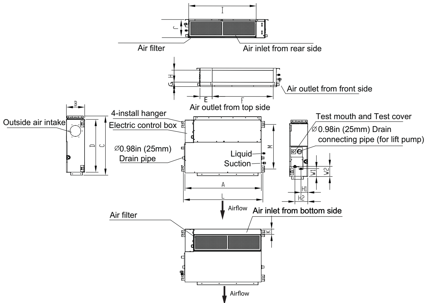
Fig. 5 — Indoor Unit Sizes 9K - 48K
