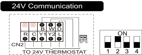
Fig. 21 —Scenario 3 - Wiring to the Outdoor Unit
