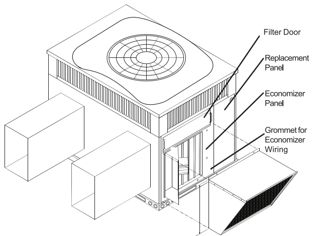
Horizontal Economizer
