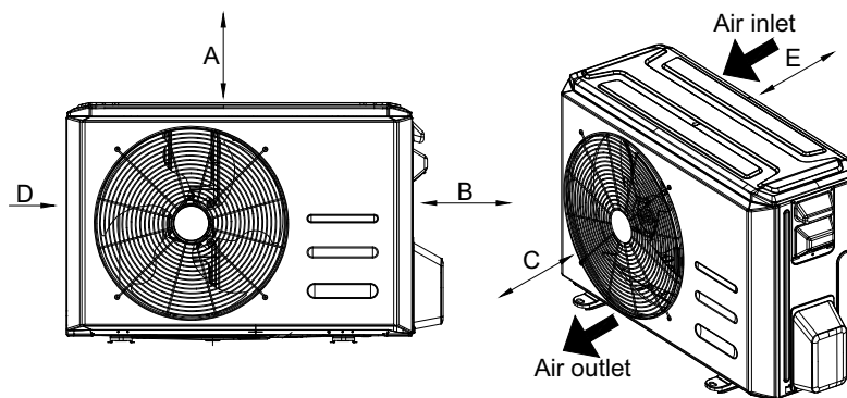
Fig. 5 – Clearances
