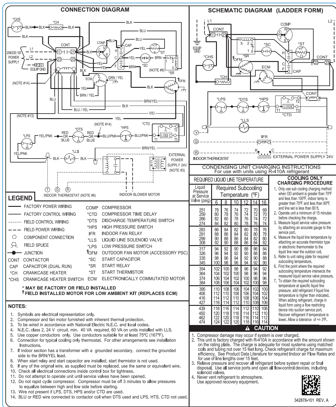
Fig. 4 – Wiring Diagram — Model BA16NW061, 208/230-1 - Legacy models, no longer in production
