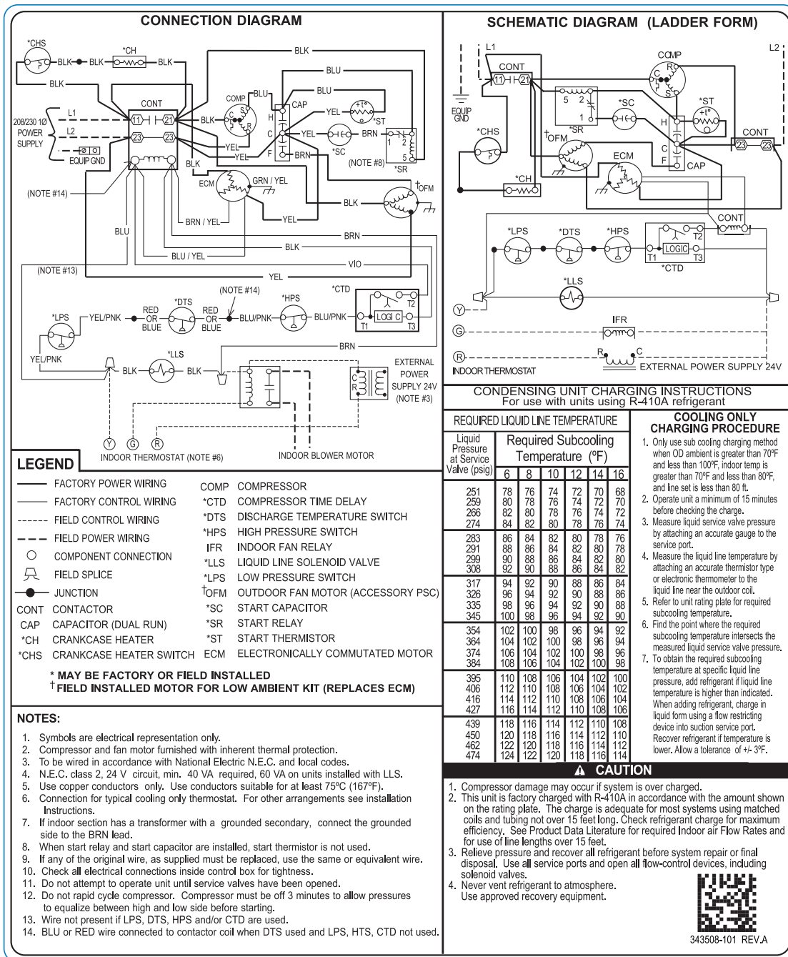
Fig. 2 – Wiring Diagram — Model BA16NW, sizes 054 and 061, 208/230-1
