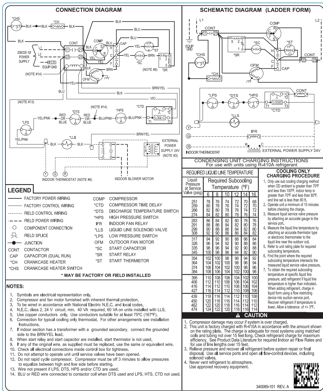
Fig. 3 – Wiring Diagram — Models BA16NA036-061, BA16NW036-060, 208/230-1 - Legacy models, no longer in production
