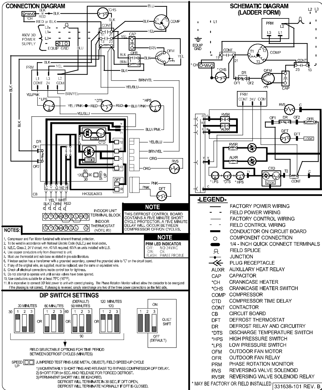
Fig. 4 – Wiring Diagram — Model sizes 36 - 60, 460-3
