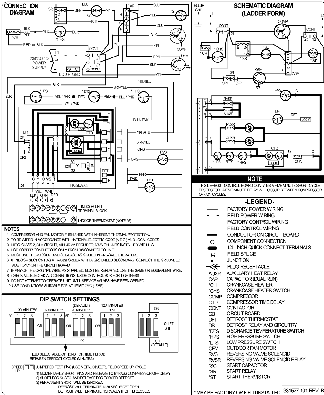
Fig. 2 – Model size 60, 208/230-1
