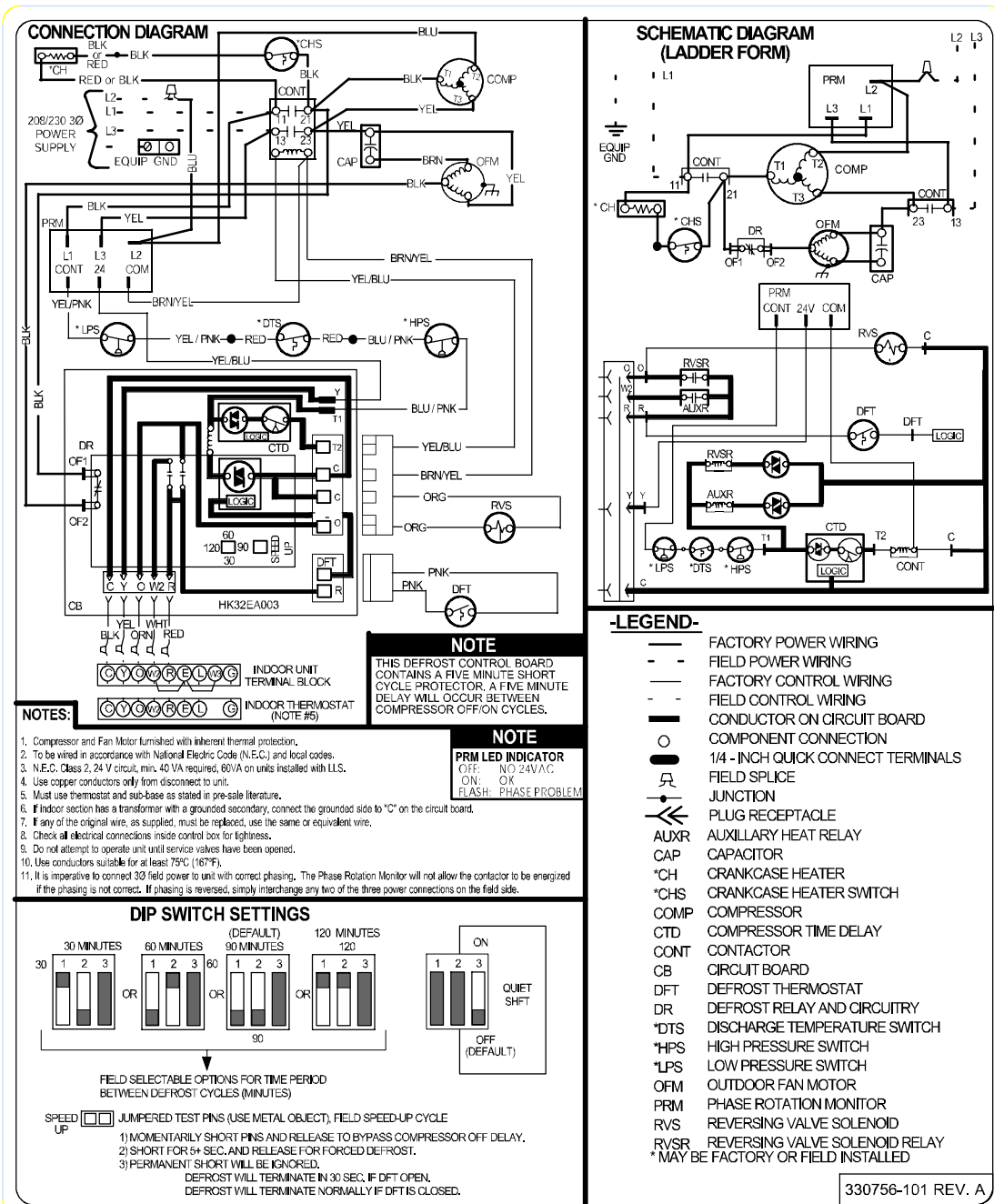
Fig. 3 – Wiring Diagram — Model sizes 30 - 60, 208/230-3
