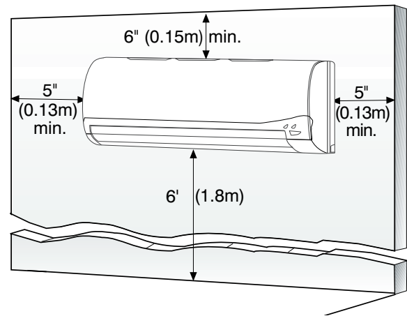
Fig. 2 – 40MVC Clearance
