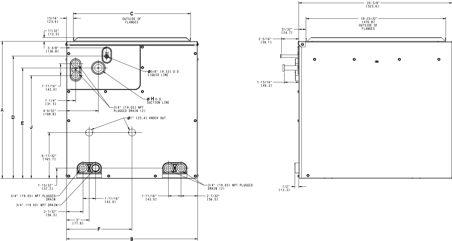
Fig. 9 – CVAMA Dimensions
