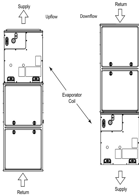
Fig. 2 – Typical Flush-Fit Coil Installation on Furnace (recommended)
