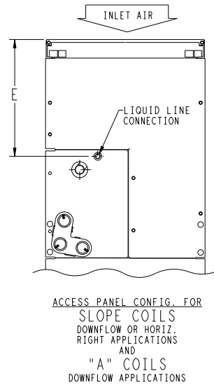
Fig. 1 – FCMA5 Dimensional Drawing, sheet 1
