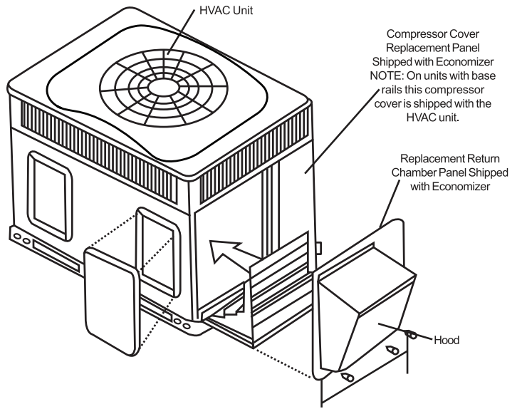
Vertical Economizer
