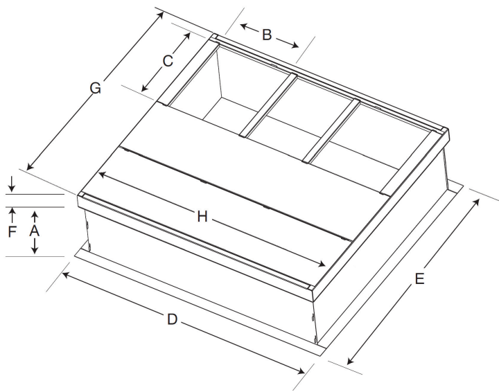
LARGE CURB
