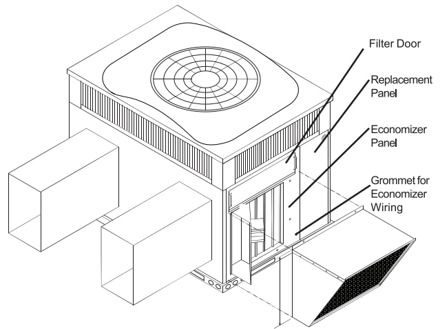
Horizontal Economizer
