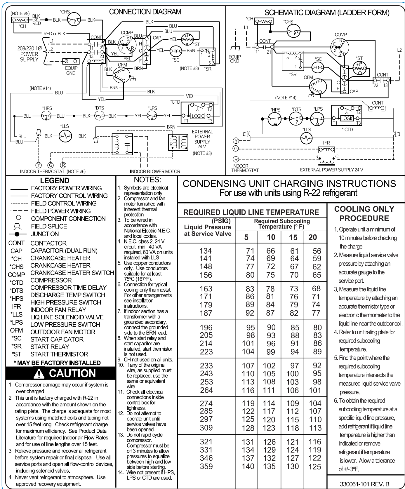
Fig. 2—PA13 060-A 208/230v, 1 Phase, 60 Hertz
