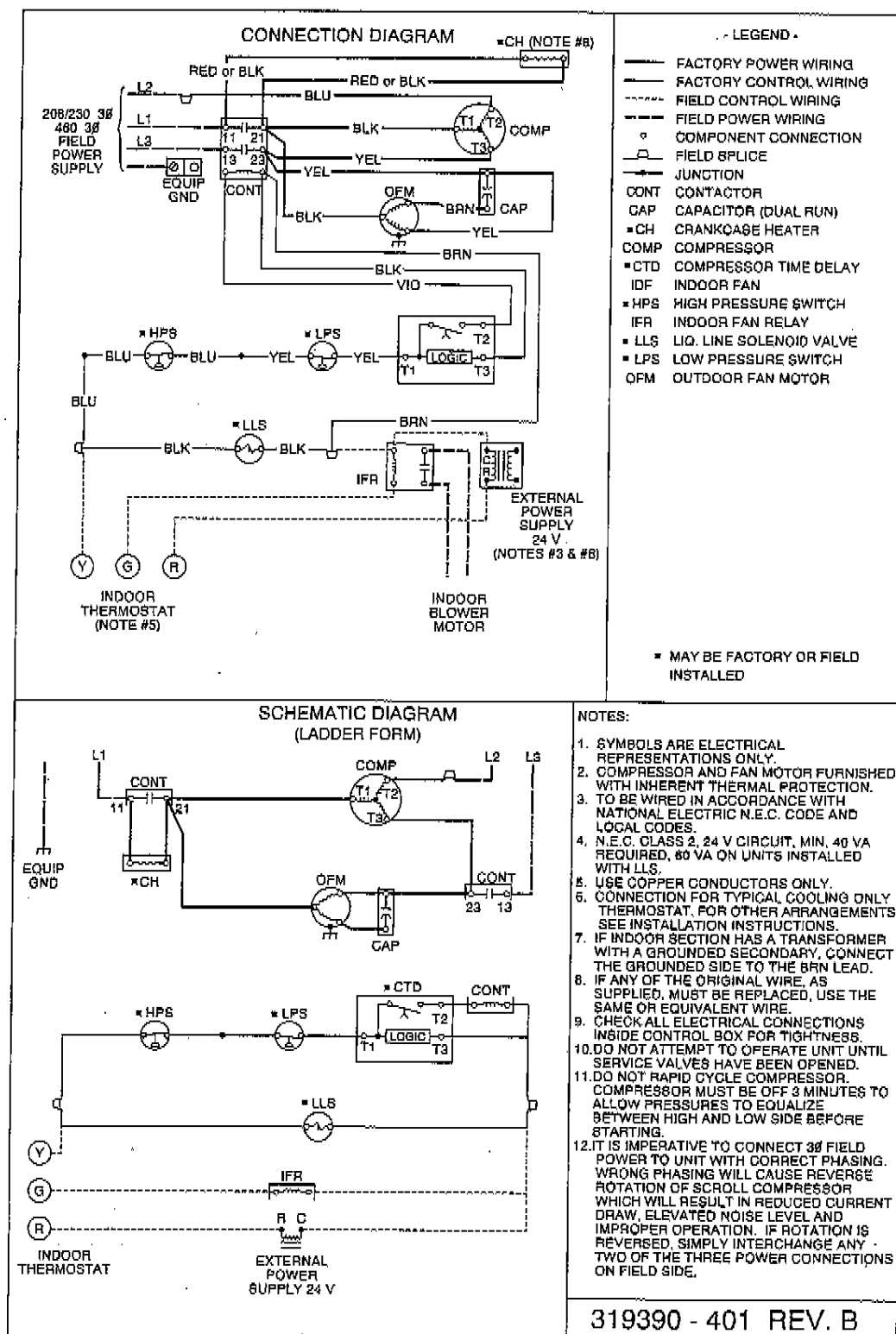
Fig. 3—38CK036-060 208/230v and 460v, 3 Phase, 60 Hertz
