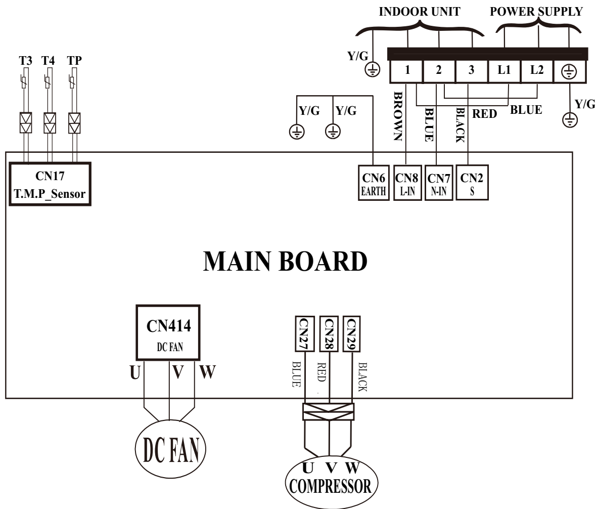
Fig. 9 — Wiring Diagram Size 24K (230V) - Cooling Only
