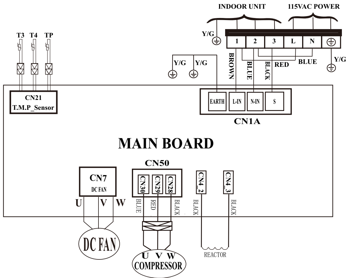
Fig. 7 — Wiring Diagram Size 12K (115V) - Cooling Only
