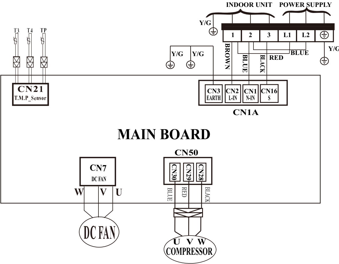
Fig. 8 —Wiring Diagram 12K/18K (208/230V) - Cooling Only
