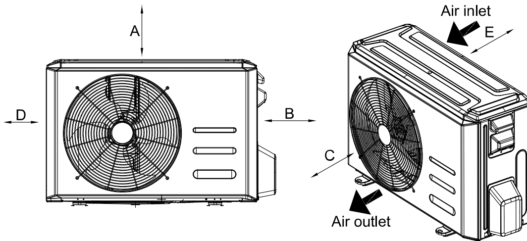
Fig. 5 — Clearances
