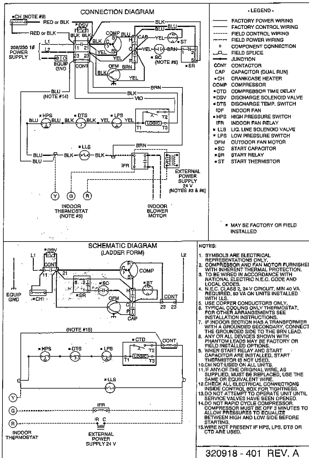
Fig. 1—38TRA024-048 208/230v, 1 Phase, 60 Hertz
