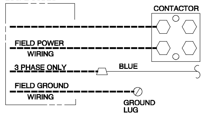
Fig. 5 - Line Connections
