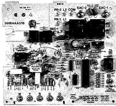
PRINTED-CIRCUIT BOARD
