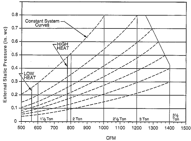
AIR DELIVERY CURVE—042040
