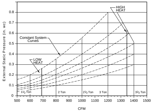
AIR DELIVERY CURVE — 042080
