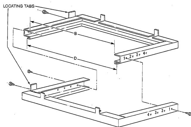
Disassembled
