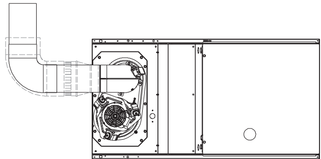
Fig. 4 - Downflow Application-Vent Elbow Left then Up
