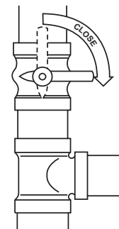
Fig. 4 – Close Valve
