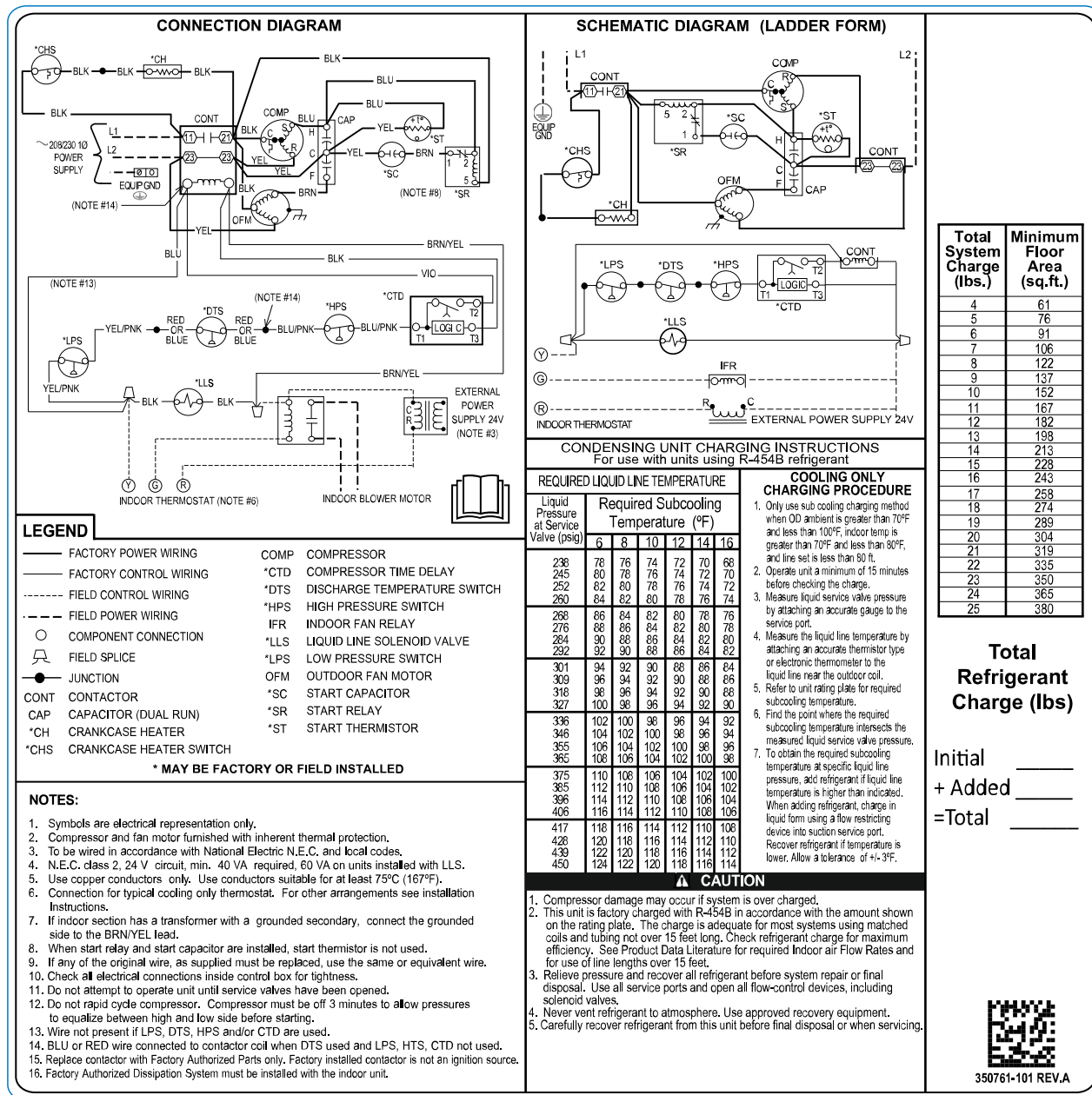
Fig. 1 – Sizes 18 - 60
